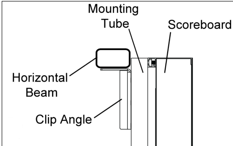
Figure 8: Mounting Tube Attachment, Side View
