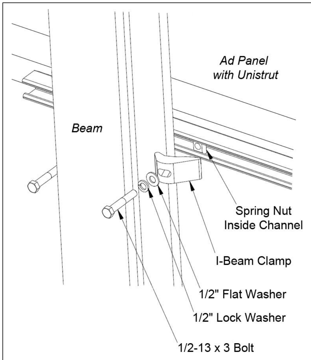
Figure 10: Ad Panel Mounting with I-beam Clamps, Rear Isometric View
