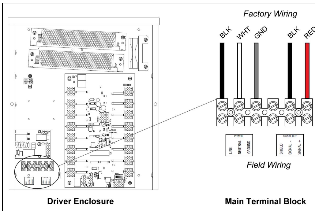
Figure 13: Driver Enclosure & Main Terminal Block
