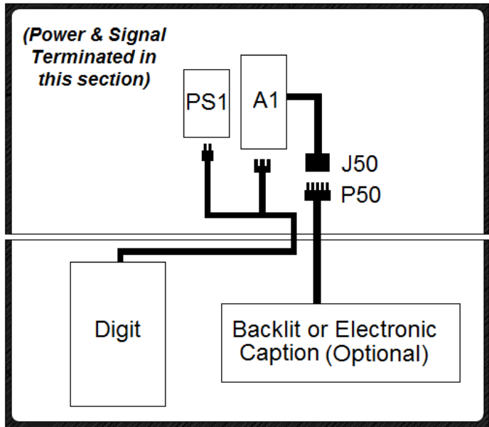
Figure 17: T.O.L. Power/Signal Interconnections (Front View)
