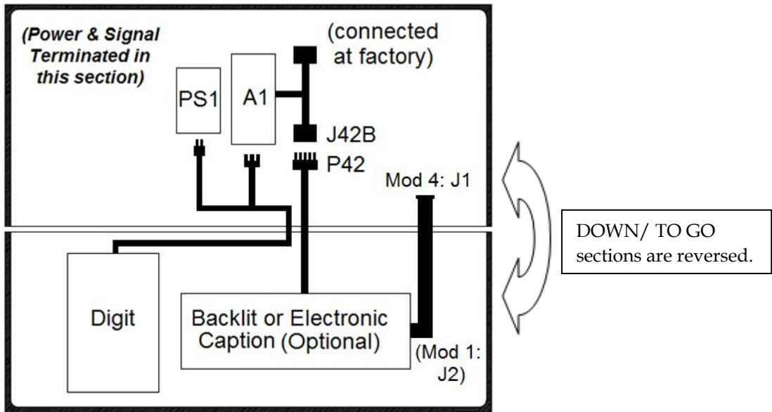
Figure 18: BALL ON/QTR Power/Signal Interconnections (Front View)
