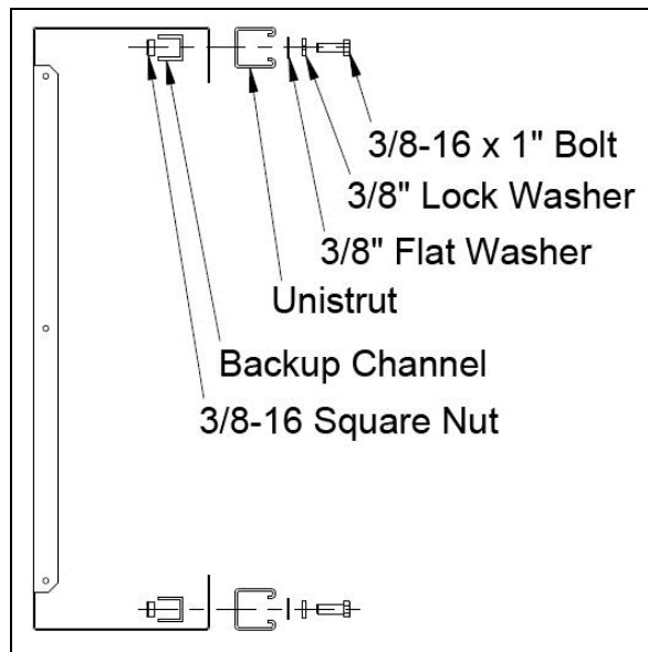
Figure 9: Unistrut Attachment, Side View
