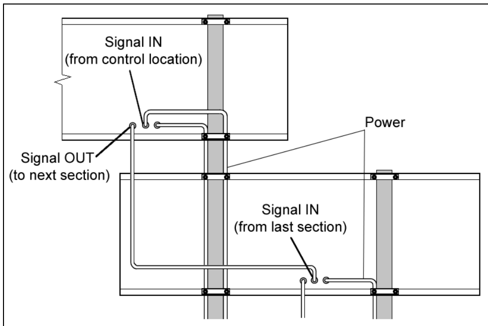
Figure 19: Re-driving Signal (Rear View)
