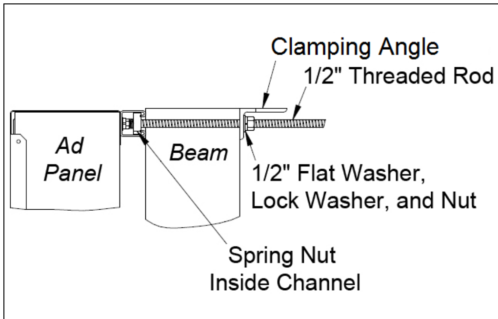
Figure 11: Ad Panel Mounting with Clamping Angles, Side View
