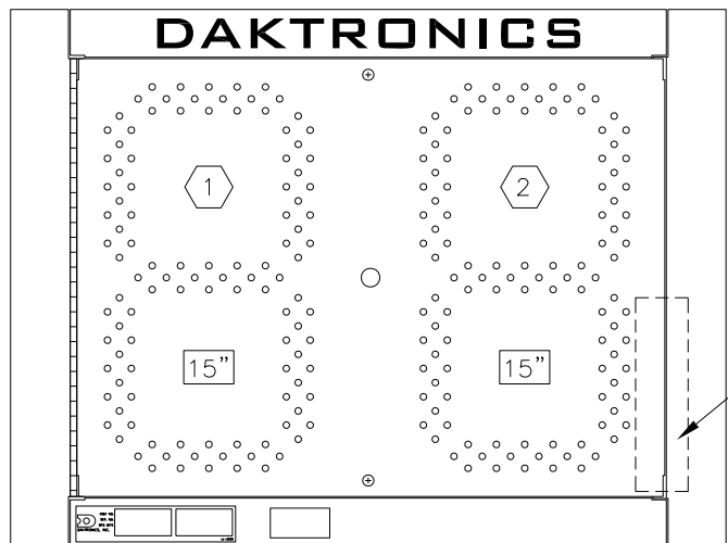
FRONT VIEW DOOR SHOWN CLOSED
