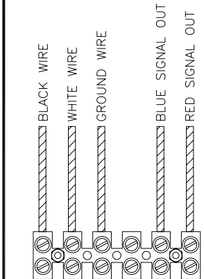
DETAIL: A (SCALE 1=1.5)
