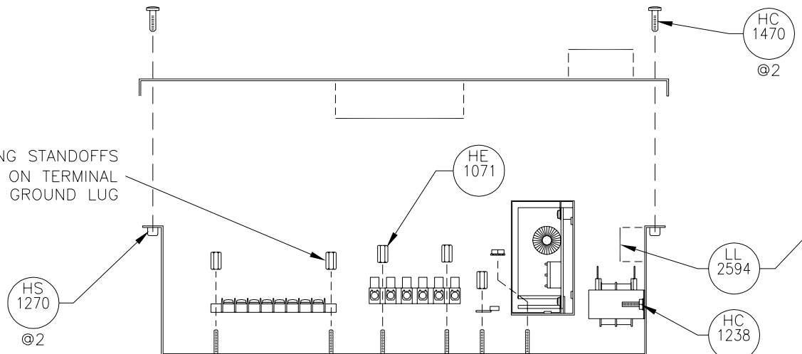
BOTTOM VIEW
