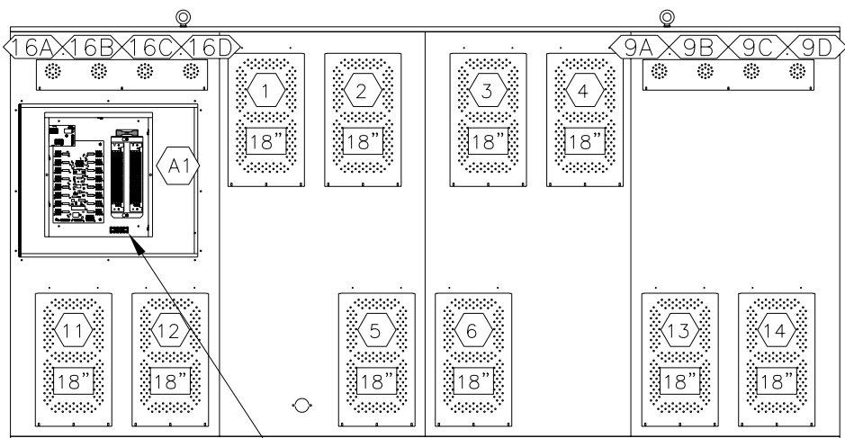
REAR VIEW
