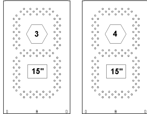
Figure 14: Digit Designation
