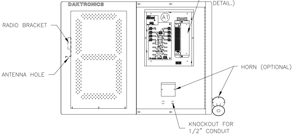
FRONT VIEW ACCESS DOOR OPEN
