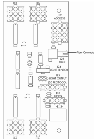
Figure 9: Driver Fiber Connection Location
