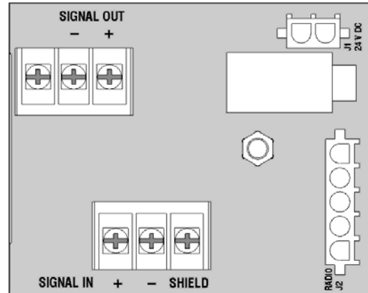
Figure 8: Signal Surge Arrester Card
