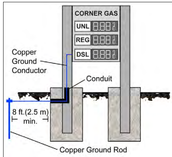
Figure 4: Correct Grounding
