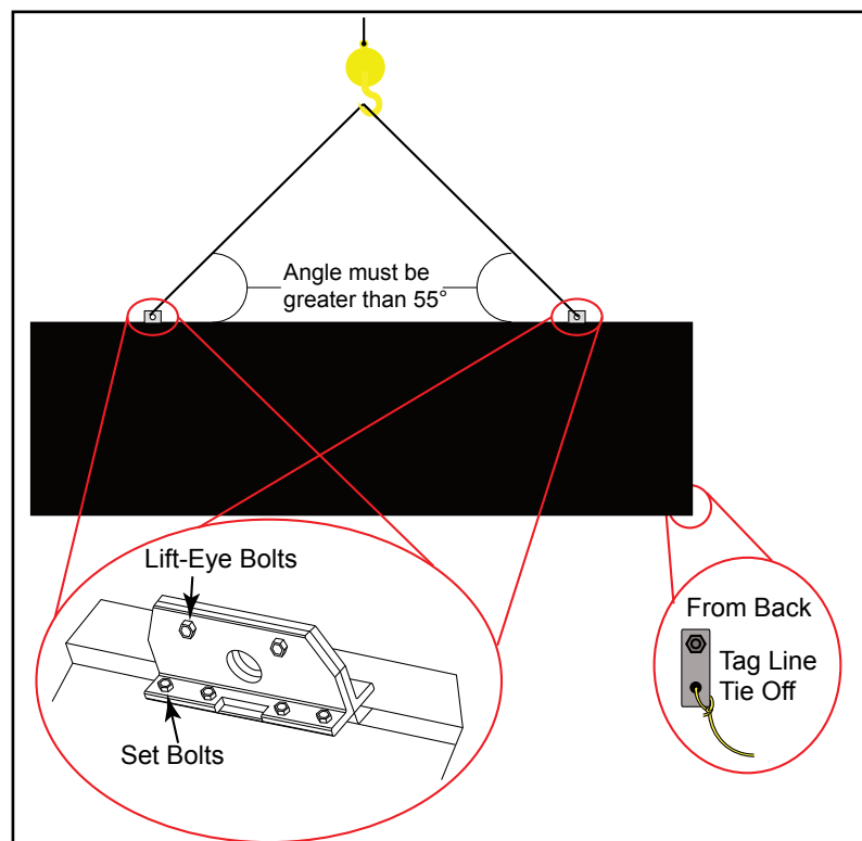
Figure 2: Proper Display Lifting
