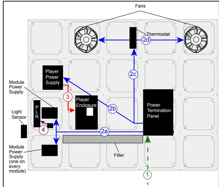
Figure 22: Power Routing
