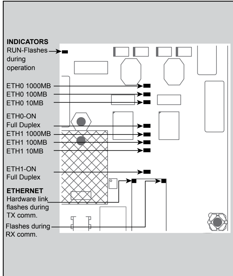
Figure 24: Controller Diagnostic LEDs
