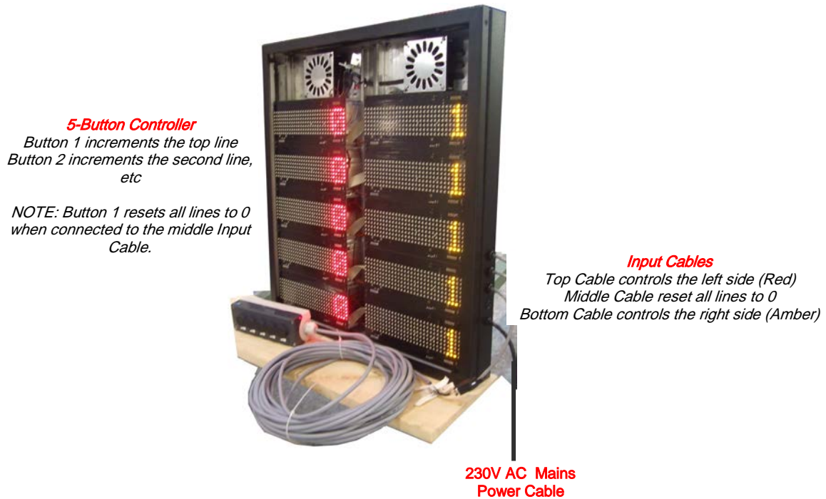
Figure 1 – System Configuration.
