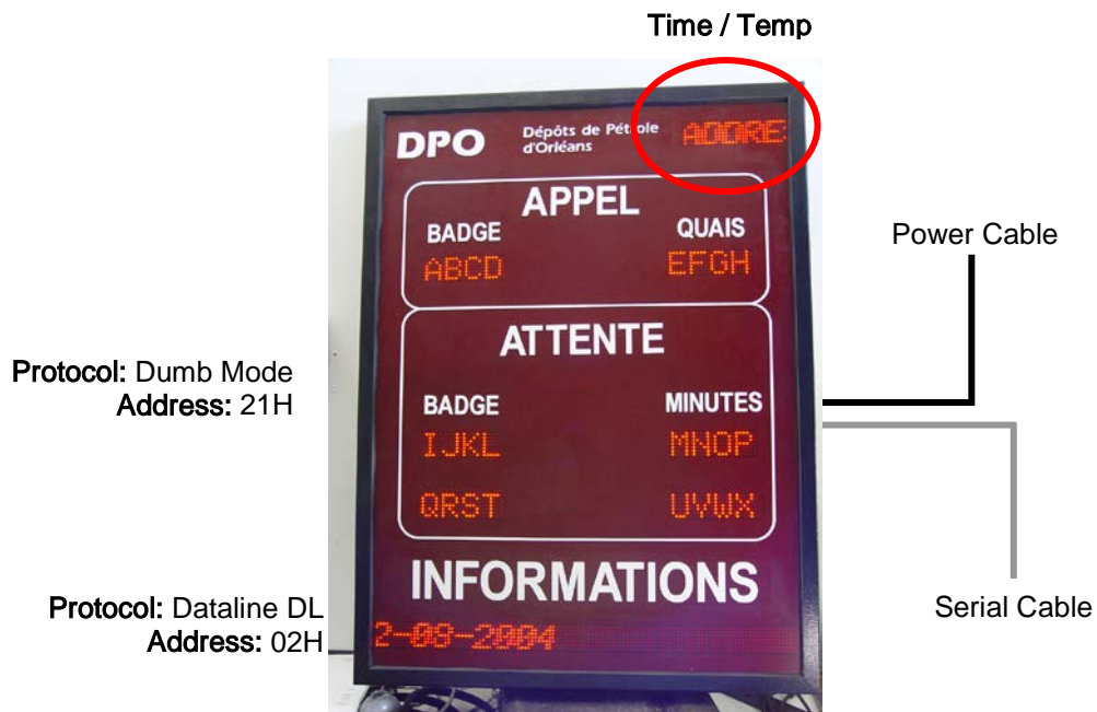
Figure 1 – System Configuration.
